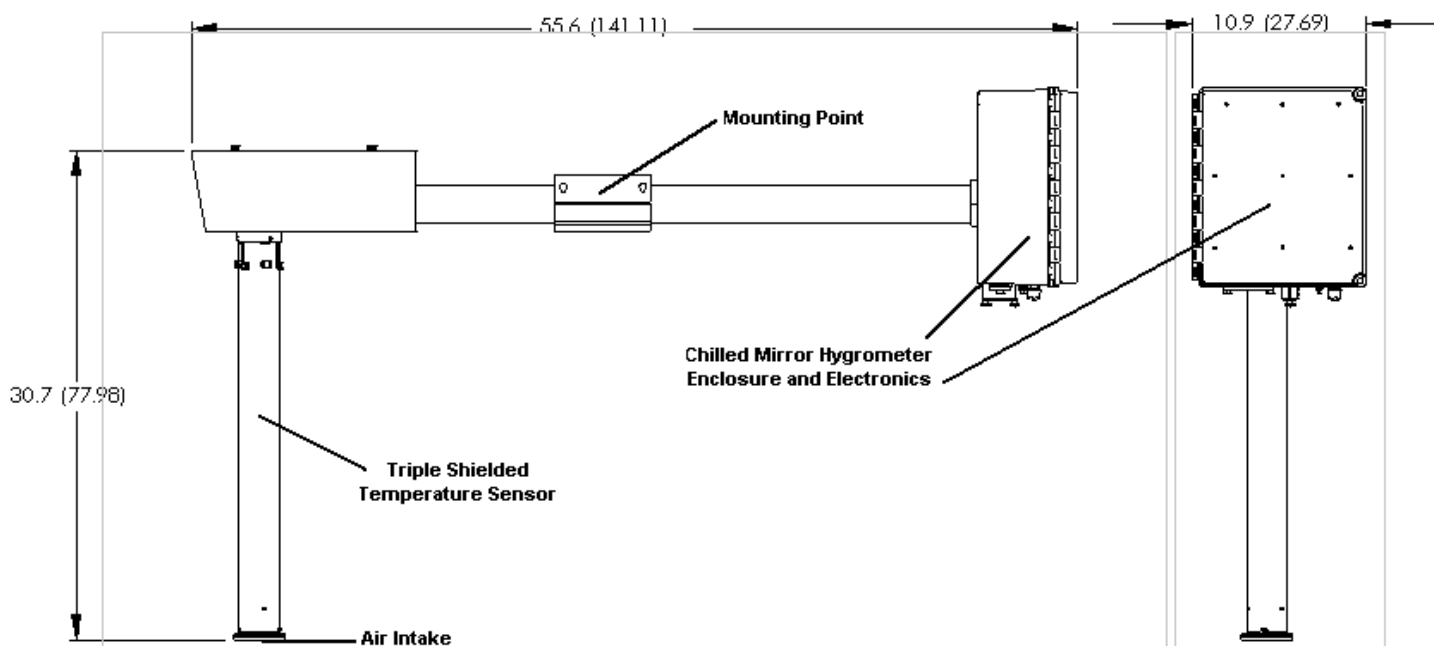
Mechanical Interface, Dimensions in inches (cm)
